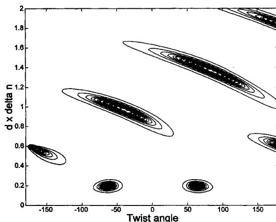
Fig. 1. Contrast ratio of the RBTN as a function of d\Delta n and \phi for \alpha = 0 . Each contrast contour line represents an increase of 3.
