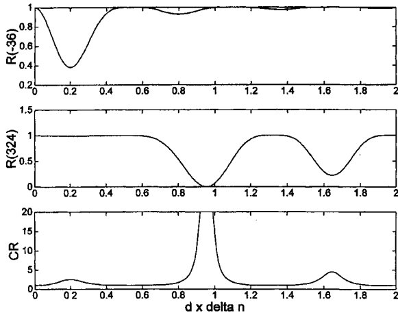
Fig. 3. Reflectance of the two bistable states (top) and the contrast ratio (bottom) as a function of d\Delta n for \phi = -36^\circ .
