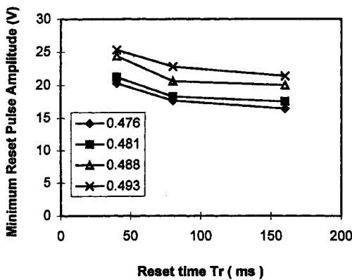
Fig. 8. Minimum reset pulse amplitude as a function of the reset time. The selection time is fixed at 1 ms.
